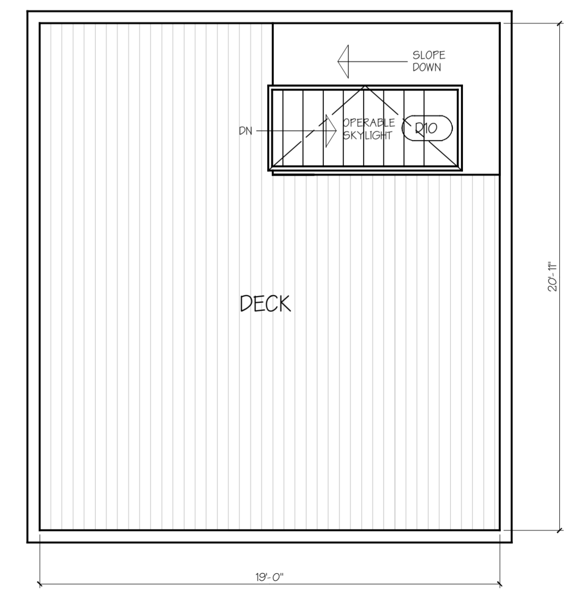
3 ROOF DECK FLOOR PLAN 1/4" = 1'-0"
