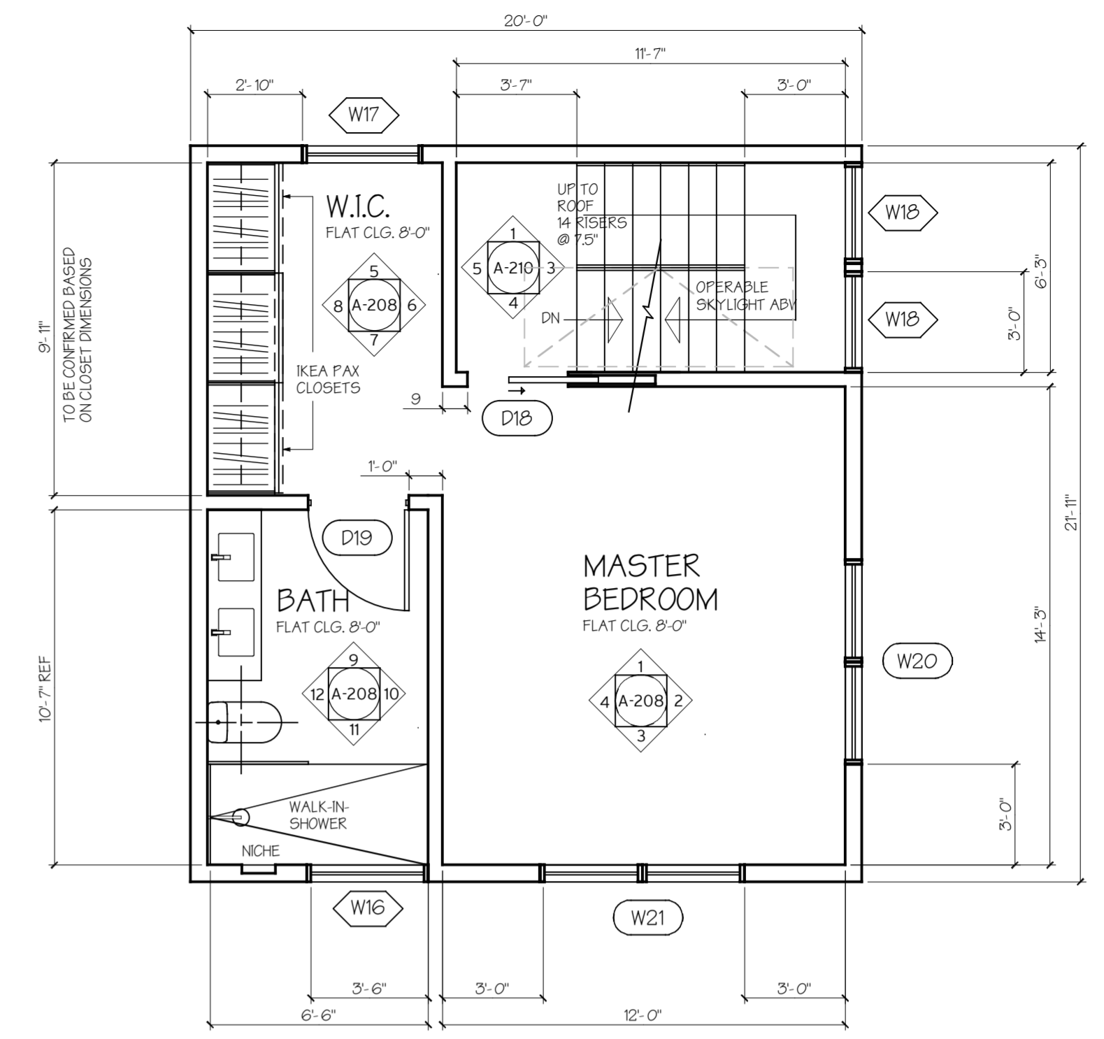
2 SECOND LEVEL FLOOR PLAN 1/4" = 1'-0"
